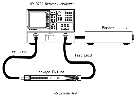
Figure 2: Shielding effectiveness test setup
